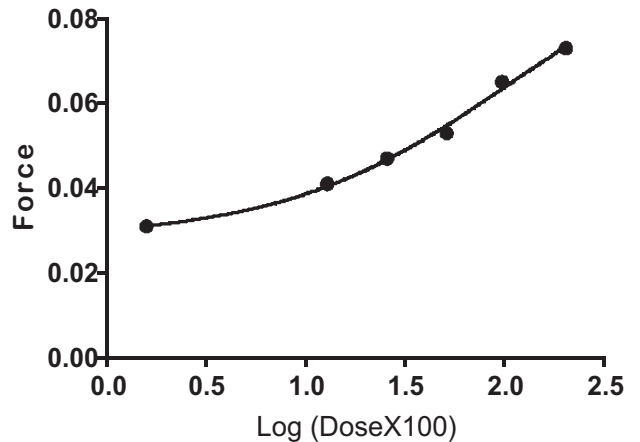
Figure 7: Modified concentration-response curve for the hot extract
